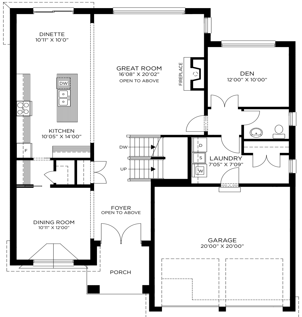
FIRST FLOOR PLAN (STANDARD)
