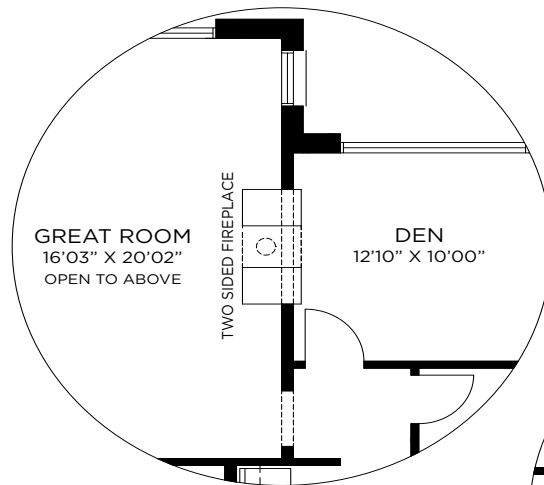
FIRST FLOOR PLAN (OPTIONAL)
