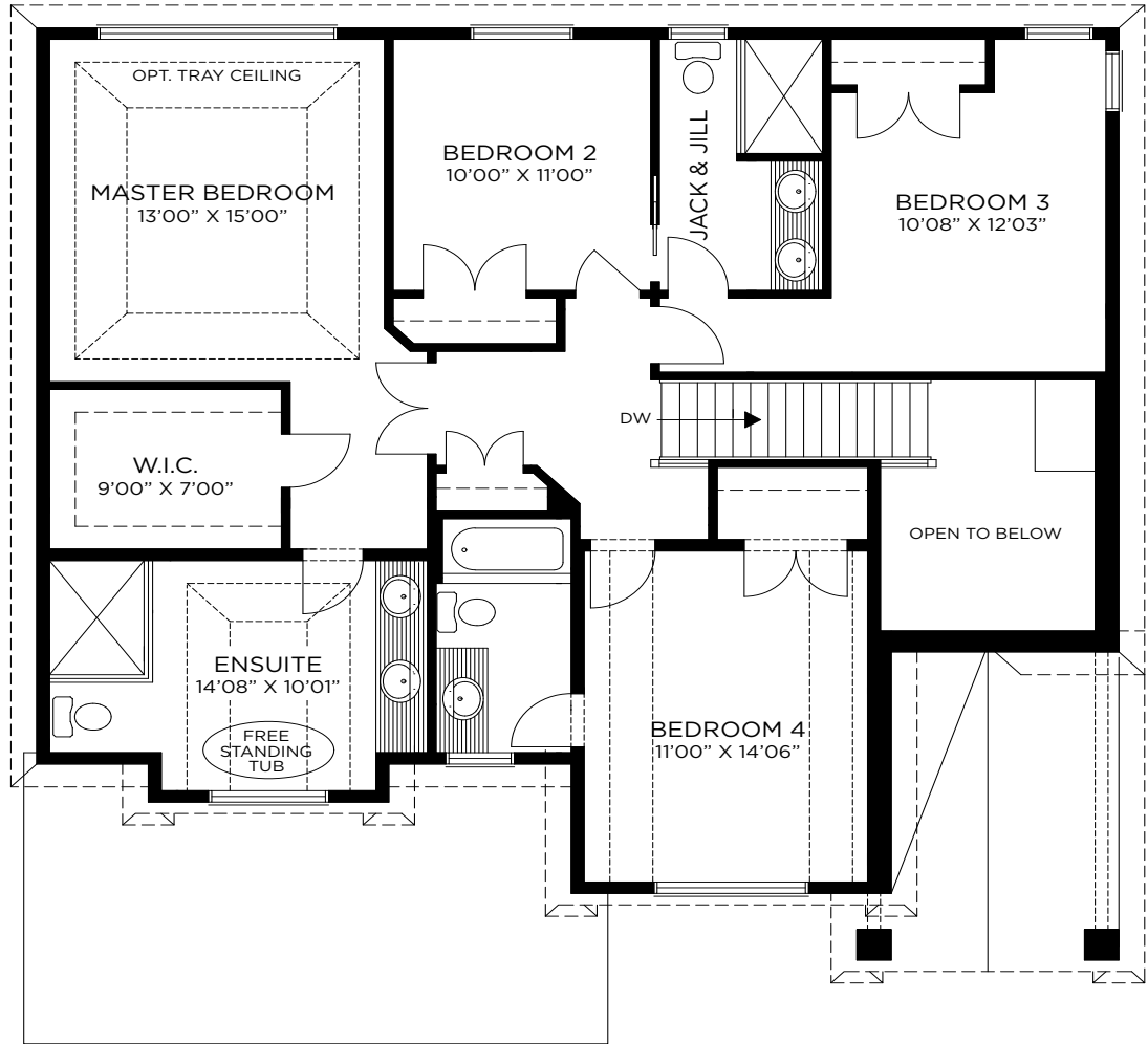
SECOND FLOOR PLAN (OPT. 1)
